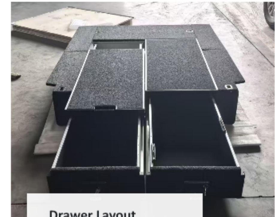
Drawer Layout
